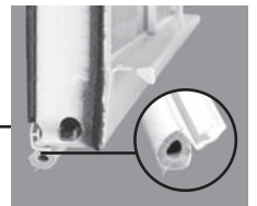
Front Load Bulb Seal: 109-22-32692-WHT-6 109-22-32692-BEI-6
